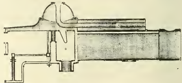
PHLEGER'S BOILER. FIG. 72.
